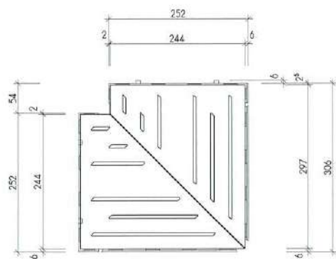
External corner
