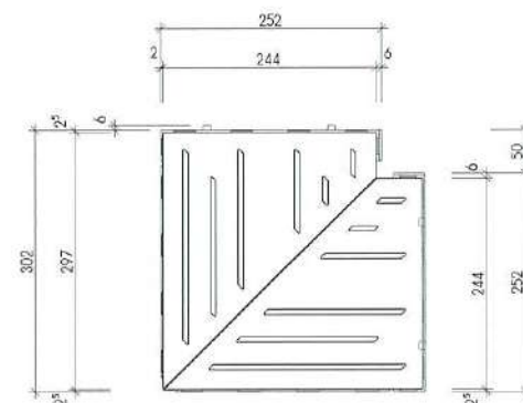
Internal corner
